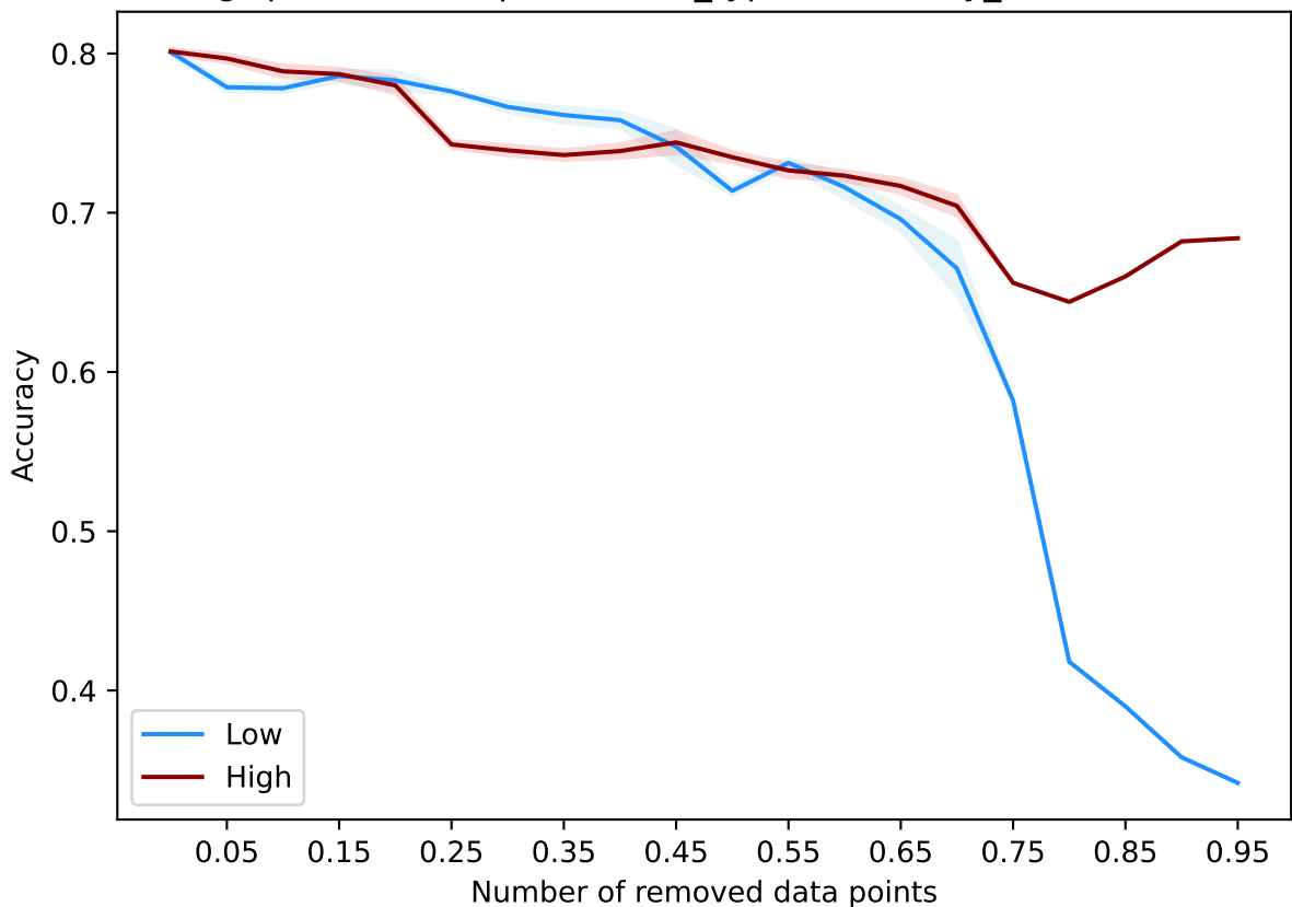
PruningOptimization(optimization_type=size, only_size=250) - adult
